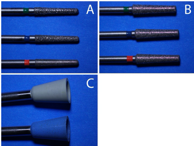
Figure 1. Grinding burs and polishing system A) Diamond grinding burs; B) Zirconia-specific diamond grinding burs; C) Zirconia-specific polishing system
